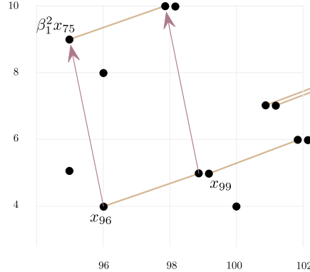
FIGURE 1. E_2^{s,f}(S) in degrees 95 \leq s \leq 102 , 4 \leq f \leq 10 . Brown lines represent \alpha_1 -multiplication. Each dot represents a copy of \mathbb{F}_3 . The information in this chart used in the proof of Lemma 3.4 is summarized in Lemma 3.1(2)(3).
