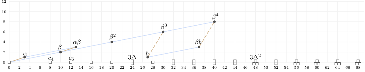
FIGURE 5. The E_\infty page of the elliptic spectral sequence computing \pi_s tmf for 0 \leq s \leq 71 . Dashed brown lines represent hidden \alpha -multiples. Squares indicate copies of \mathbb{Z}_3 and dots indicate copies of \mathbb{F}_3 .
