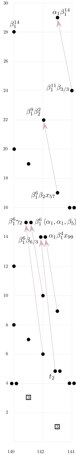
FIGURE 3. E_2^{s,f}(S) in degrees 140 \leq s \leq 144 , along with some Adams-Novikov differentials. A box containing “3” denotes a copy of \mathbb{Z}/27 . Multiplications by \alpha_1 are not shown.
