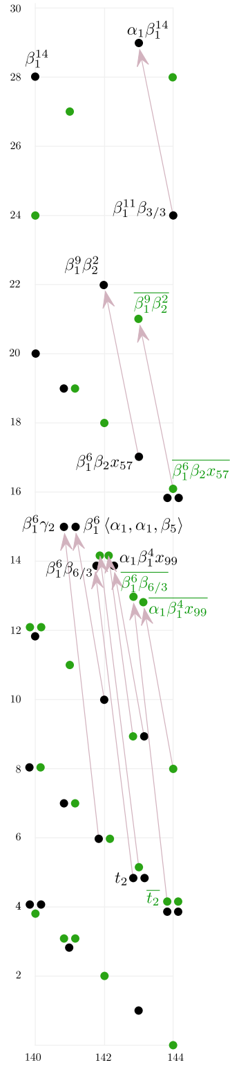
FIGURE 4. E_2^{s,f}(S/3) in degrees 140 \leq s \leq 144 , along with some Adams-Novikov differentials. Green dots denote top cell classes. Multiplications by \alpha_1 are not shown.
